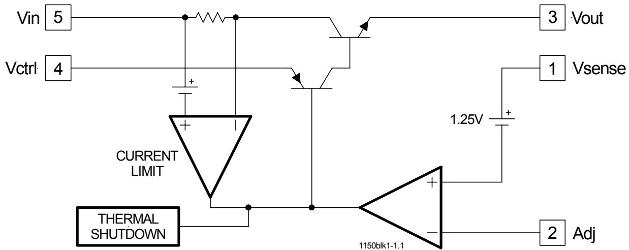
Figure 2 - Simplified block diagram of the IRU1150
