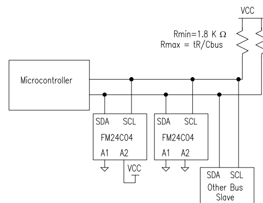
Figure 2. Typical System Configuration
