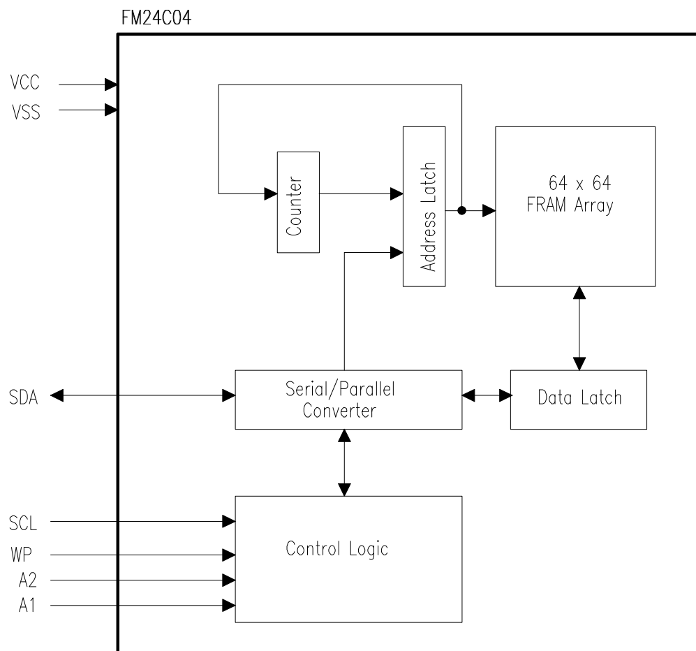
Figure 1. Block Diagram
