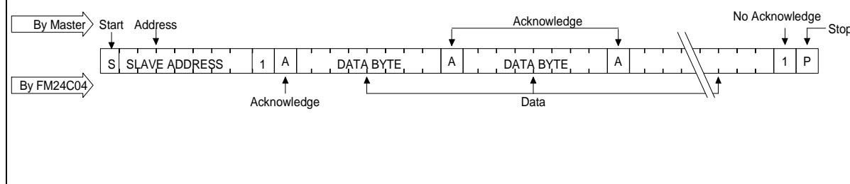
Figure 8 Sequential Read
