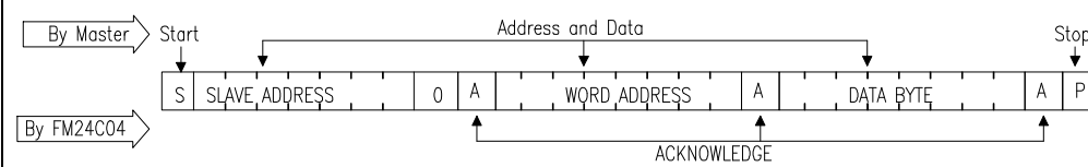
Figure 5 Byte Write
