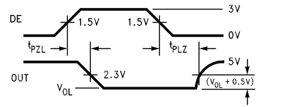
FIGURE 10. TRI-STATE Waveforms ( t_{pZL} , t_{pLZ} )
