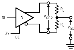
FIGURE 1. Driver V_{OD2} and V_{OC}
