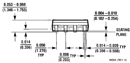
8-Lead (0.150" Wide) Molded Small Outline Package, JEDEC Order Number DS36C278TM, DS36C278M NS Package Number M08A
