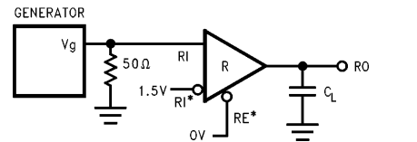
FIGURE 12. Receiver Differential Propagation Delay Test Circuit
