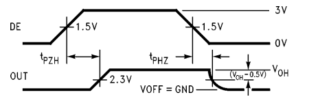
FIGURE 8. TRI-STATE Waveforms ( t_{pZH} , t_{pHZ} )
