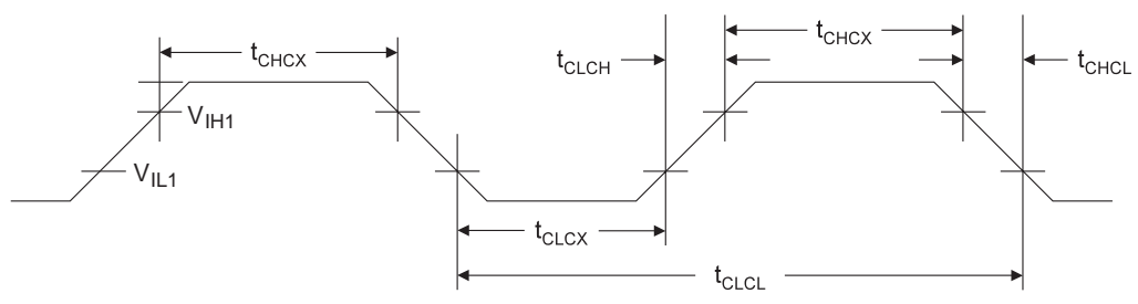
Figure 126. External Clock Drive Waveforms
