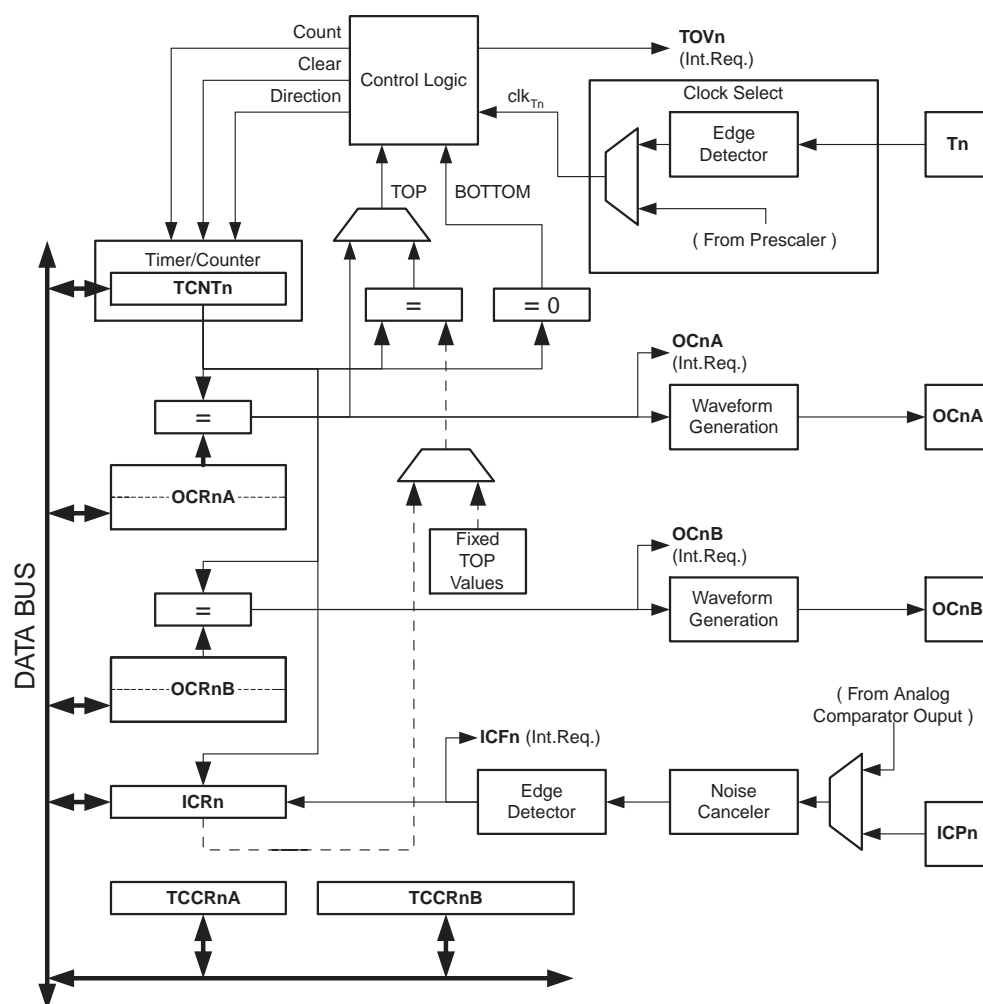
Figure 40. 16-bit Timer/Counter Block Diagram (1)
