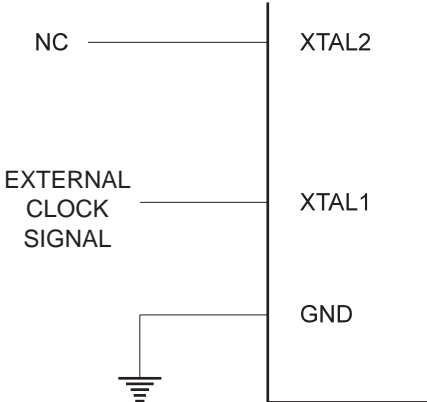
Figure 14. External Clock Drive Configuration
