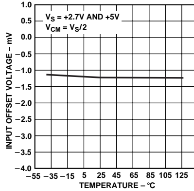
Figure 2. Input Offset Voltage vs. Temperature
