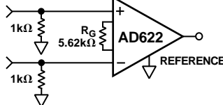
AD622 Monolithic Instrumentation Amplifier, G = 9.986
